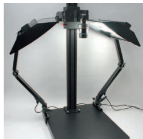
Variable lens perfect for documentation of big samples with incident illumination
