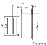
DALSA Piranha 3 Mount
