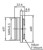
Nikon F Mount
