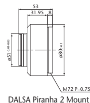
DALSA Piranha 2 Mount
