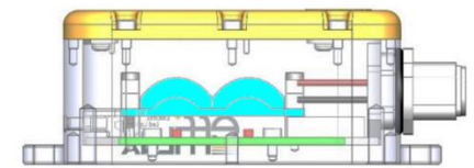
P1: screw+spacer+spacer+lens
