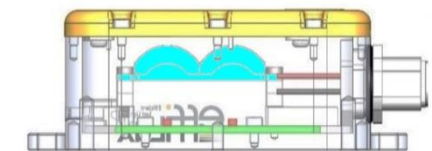
P3: screw+lens+spacer+spacer
